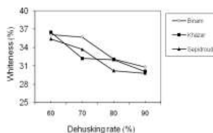
Fig. 6. Effect of dehushing rate on the rice whiteness of different varieties
