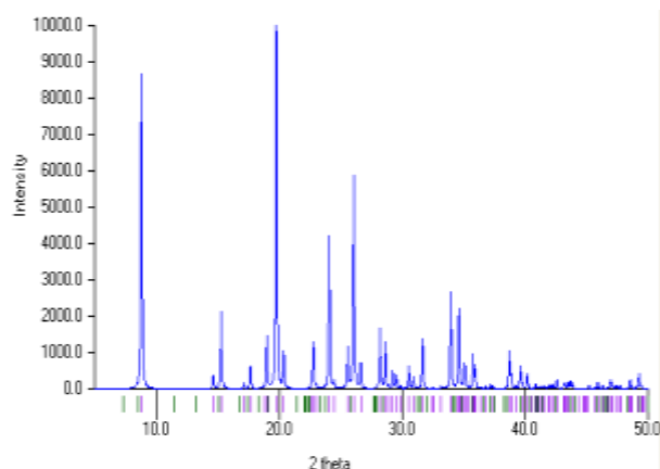
Fig 3. X-ray diffraction pattern of L-Proline Monohydrate
