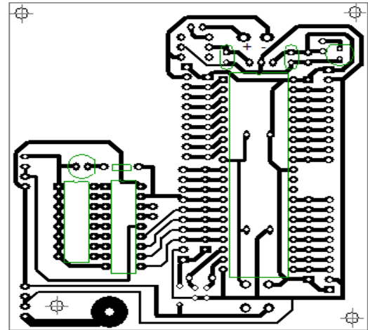
Figure 6. PCB design of microcontroller and receiver section
