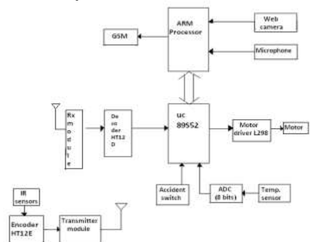
Figure 1. Block diagram of Car black-box
