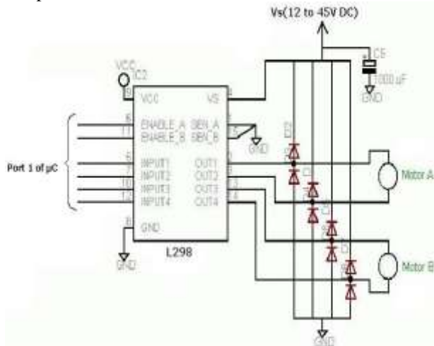
Figure 5. Working of Motor driver L298
