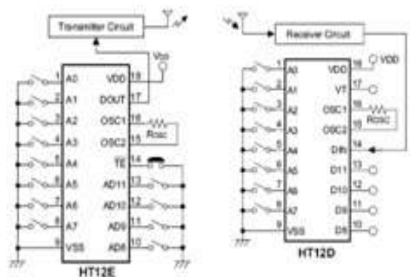
Figure 4. Encoder and Decoder assembly
