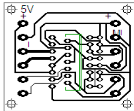
Figure 7. PCB design of motor driver section
