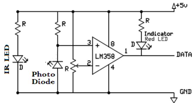
Figure 3. Working logic of IR sensors
