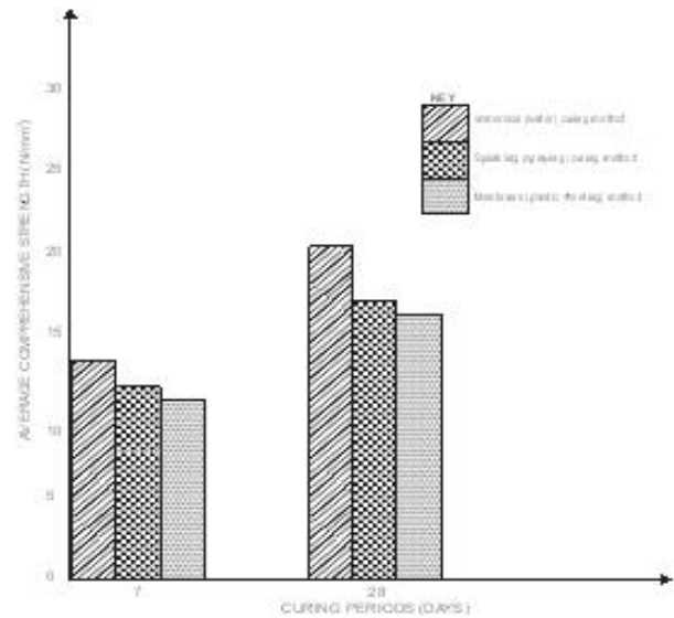
Fig 3: Graph of average compressive strength versus curing ages for Different methods of curing used in the experiment
