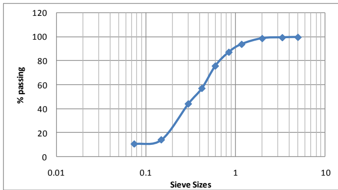
Fig 2: Particle Distribution Curve for Fine Aggregate
