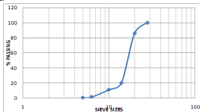
Fig 1: Particle size distribution curve for crushed granite stone
