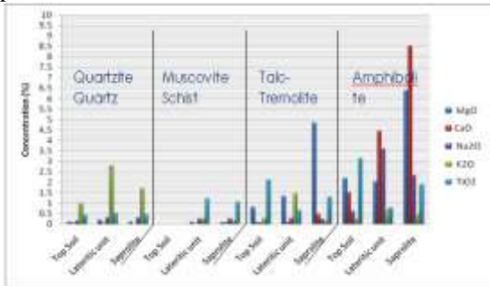
Figure 4: Histogram showing the abundance of the major oxides in the weathered profile of each bedrock.
