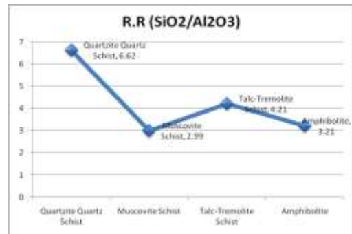
Figure 6 Plot of the Ruxton Ratio of the soil profiles. Hydrochemical Analysis
