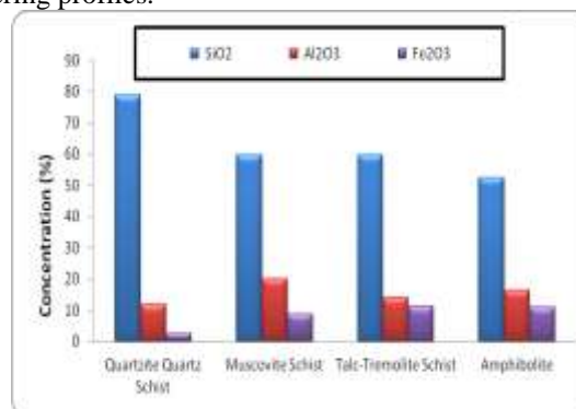
Figure 3 Mean compositions of \text{SiO}_2 , \text{Al}_2\text{O}_3 , and \text{Fe}_2\text{O}_3 in the weathering profile
