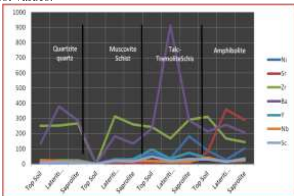
Figure 5 Plot of trace elements in the soil profile
