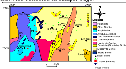
Figure 1: Geological map of the study area (Elueze, 1982) showing the sample points, P1, P2, P3, and P4, representing, quartzite quartz schist, muscovite schist, talc-tremolite schist and amphibolite respectively.
