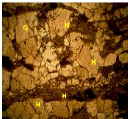
Plate 1: Photomicrograph of Amphibolite (plane polar); hornblende (H), foliated and occur as a porphyroblast within an inequant granular matrix
