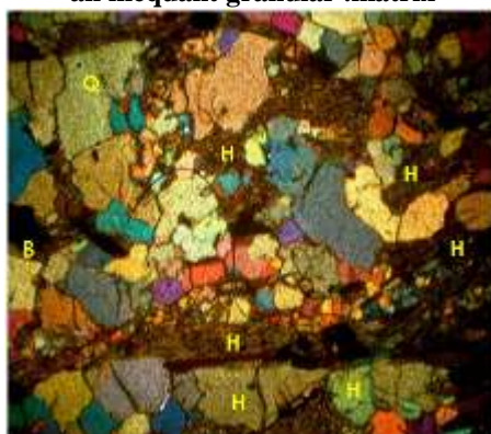
Plate 2: Photomicrograph showing the cross polar of amphibolite in thin section. Others minerals are Quartz (Q), Plagioclase (P), Biotite (B).
