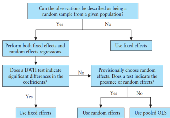
Figure 1: Choice of regression model for panel data.
