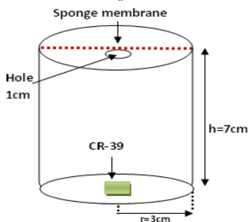
Fig.2: Schematic diagram of the optimum Radon.
