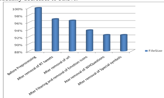
Figure 3: Comparision of file size with pre-processing techniques
