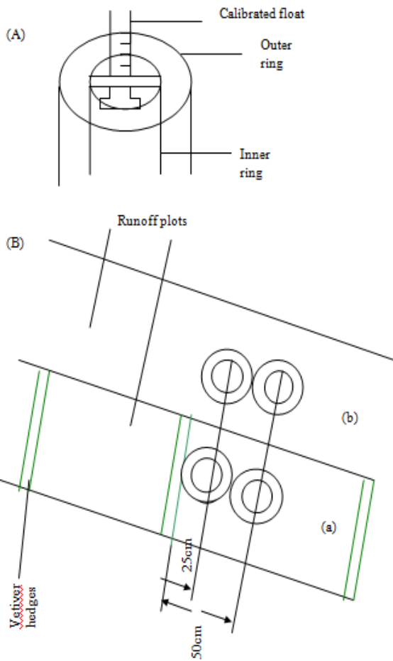
Plate 1. A diagram showing the double ring infiltrometer (A) and (B) the location of Double-Ring Infiltrometer on the (a) vetiver plot and (b) non-vetiver plot
