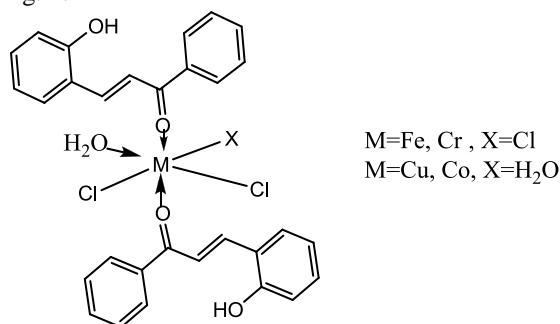
Fig. 1. Suggested structure of the prepared complexes
