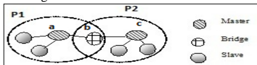
Figure 1 Scatternet Structure
