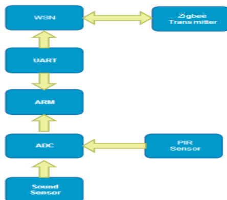
Figure 2: Transmitter Section 2
