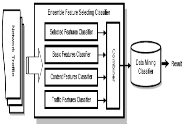
Figure 1. Hybrid intrusion detection model
