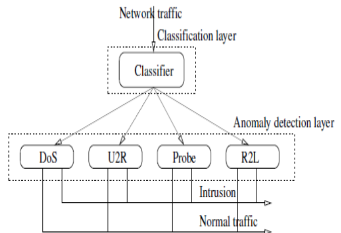
Fig 2. Authors [7] Proposed Octopus IDS Architecture
