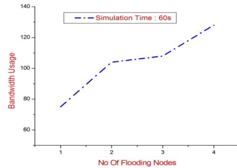
Figure 4. Number of Flooding Nodes vs. Bandwidth Usage
