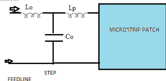
Fig 1. Circuit Diagram of Microstrip Feed
