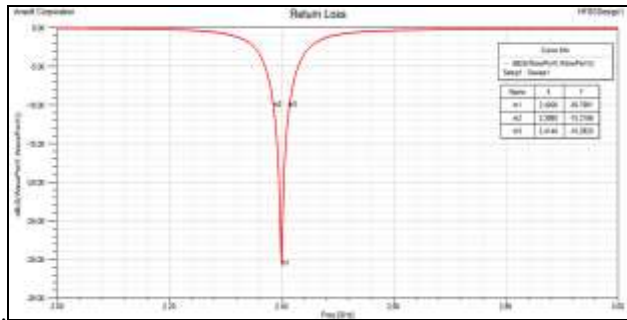
Fig 3. S- parameter plot for Return Loss v/s frequency Radiation Pattern Plots
