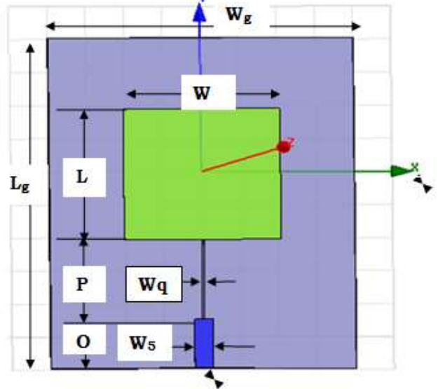
Fig: 2 Rectangular Microstrip Patch Antenna with Line Feed
