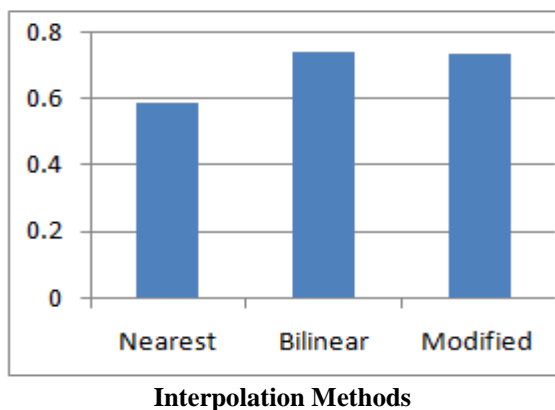
Fig 5 Graph of SSIM for different Interpolation Algorithm
