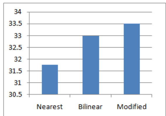
Fig. 4 Graph of PSNR for different Interpolation Algorithms
