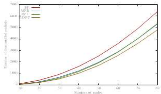
Figure 3. Comparison of OLSR and non-OLSr message diffusion techniques. We can remark that Total-Dominant Pruning Tree gives the best result, while the Partial-Dominant Pruning tree is equivalent to MPR
