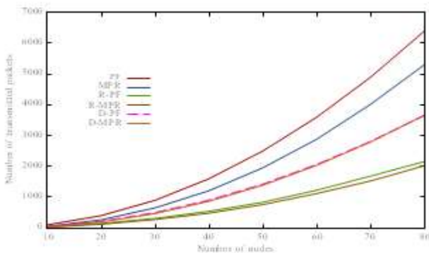
Figure 2. Comparison of existing solutions for OLSR. Observe how random network coding performs better than the deterministic one, whatever the technique it is associated to
