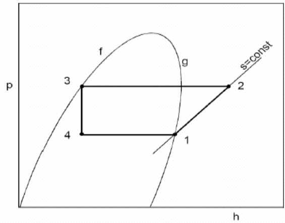
Figure 14. Refrigeration cycle
