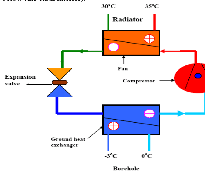
Figure 2. Detail of the GSHP circuit.
