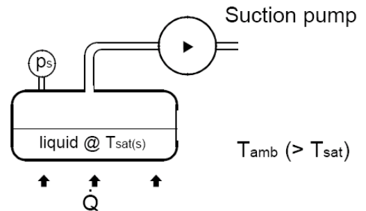
Figure 4. Refrigeration Cycle.
