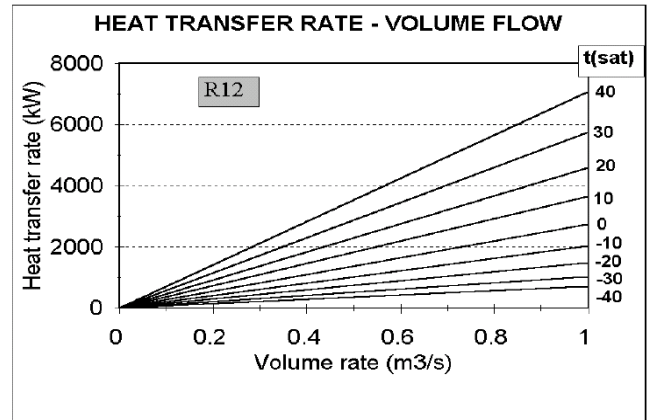
Figure 5. Heat transfer rate versus volume rate.
