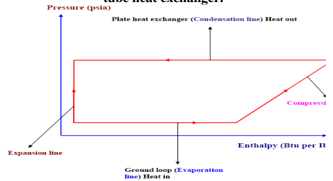
Figure 12. The ideal cycle on Pressure-Enthalpy diagram.
