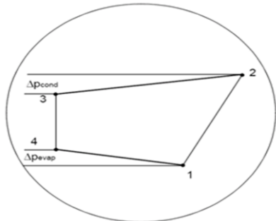
Figure 18. Pressure drops in evaporator and condenser.
