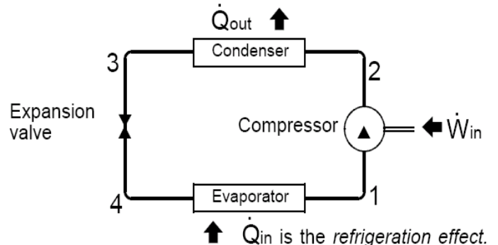
Figure 7. Simplified refrigeration system diagram
