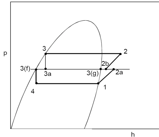
Figure 21. Cycle of multiple compressions using flash chamber
