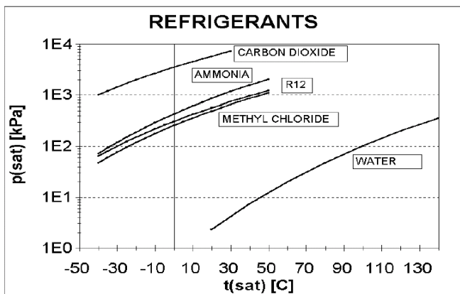
Figure 9. Refrigerant chart.
