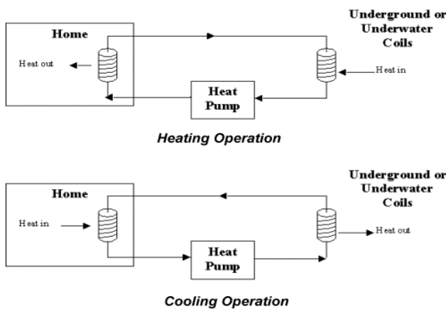
Figure 10. Heating and cooling operations.
