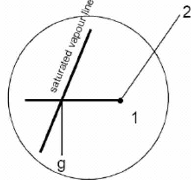
Figure 15. Evaporator superheat
