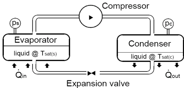
Figure 8. Heat pump refrigeration cycle.
