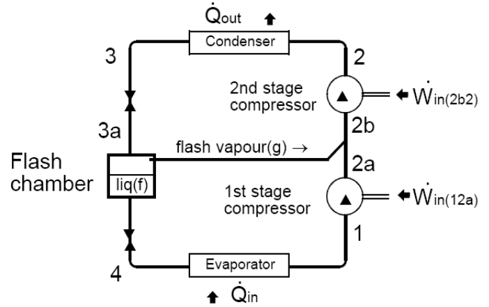
Figure 20. Liquid-suction heat exchanger cycle. Multiple Compression Using Flash Chambers
