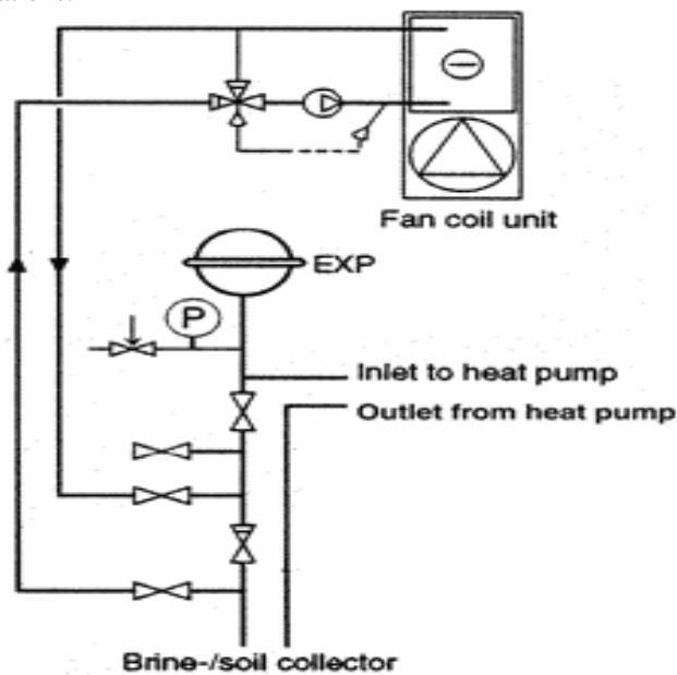
Figure 3. Diagram of cooling system.
