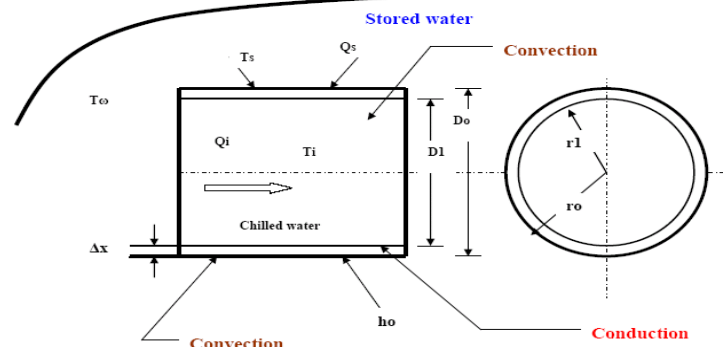
Figure 11. Schematic of heat transfer through a circular tube heat exchanger.
