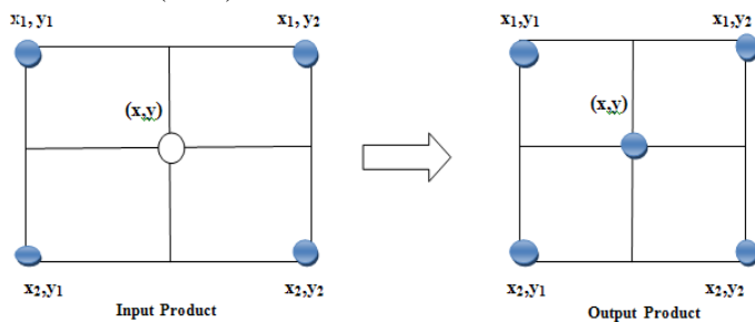
Fig 2 Bilinear Interpolation
