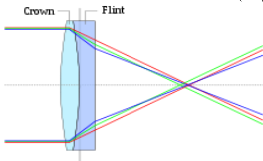
Fig. 2.1. Light rays through an achromatic lens (King, 1955)
