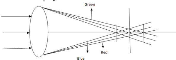
Fig. 1.4. The longitudinal chromatic aberration
