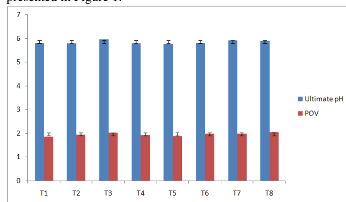
Figure 1: peroxide values (POV) and ultimate pH (pH u ) of the muscles
