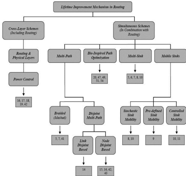
Figure 2. Classification of fundamental lifetime improvement mechanisms in routing protocols for WSNs.
