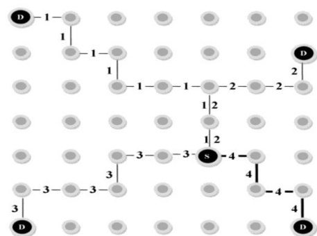
Figure 3. Path selection with minimum hop count [5].
