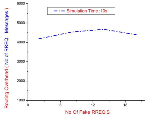
Figure 1. Number of Fake RREQs vs. Routing Overhead
