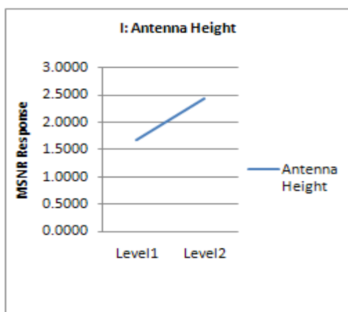
Fig 8. Antenna height Performance
