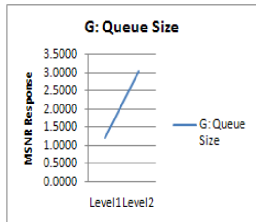
Fig 9. Queue Performance
