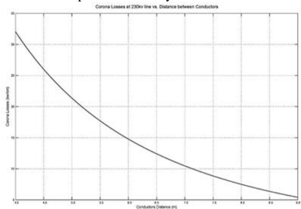
Fig 4. Corona Losses at 230 KV Line vs. distance between conductors
