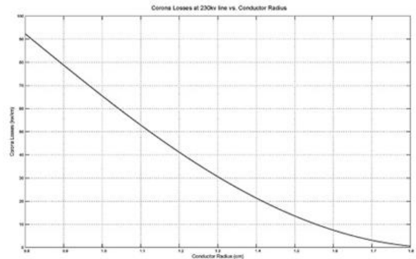
Fig 6. Corona Losses at 230 KV vs. conductor radius
