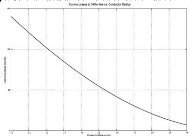
Fig 7. Corona Losses at 345 KV Line vs. Conductor Radius
