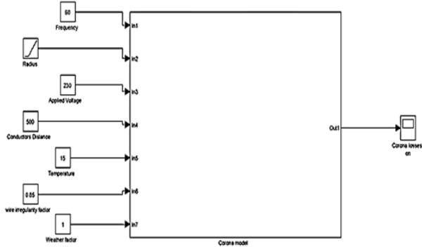
Fig 2. Developed Corona Model
