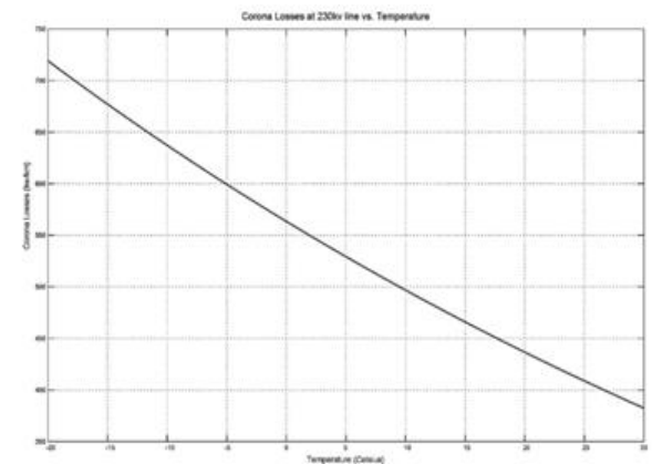
Fig 5. Corona Losses at 230 KV vs. Temperature Ambient Conditions
