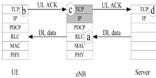
Fig. 1. The proposed congestion control mechanism
