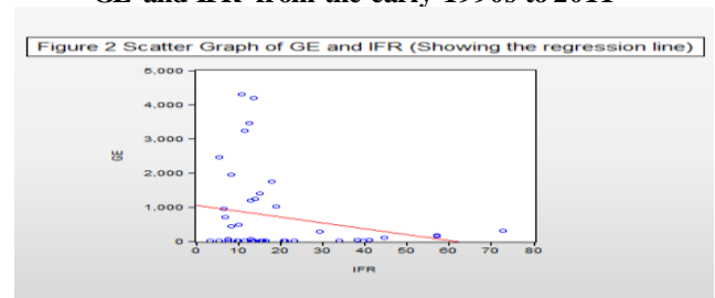
Figure 2. shows weak relationship between GE and IFR and an inverse/negative relationship is indicated by the regression line
