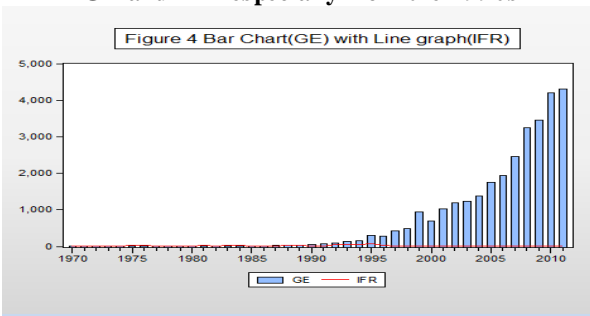
The mixed Bar Chart of GE and line graph of IFR show weak and inverse/negative relationship between GE and IFR
