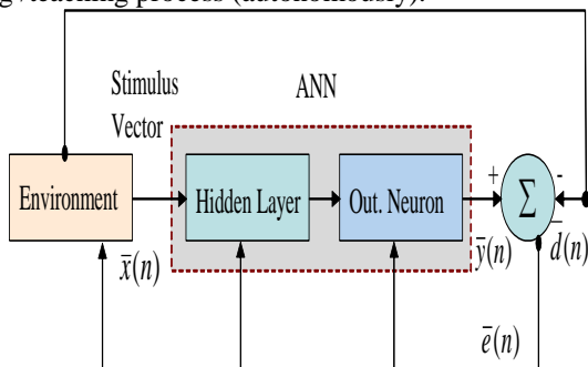
Fig 1. Basic learning/teaching ANN block diagram model for simulating realistic of learning paradigms (adapted from [15])
