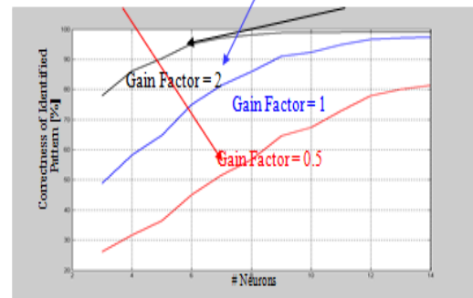
Fig 6. Illustrate students' learning achievement for different gain factors and intrinsically various number of highly specialized reading neurons which measured for costant learning rate value = 0.3.
