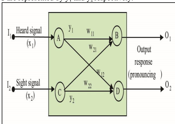
Fig 4. Generalized reading model which presented as pronouncing of some word (s) considering input stimuli and output responses
