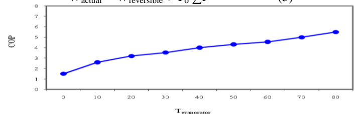
Figure 6. Heat pump performance vs evaporation temperature.
