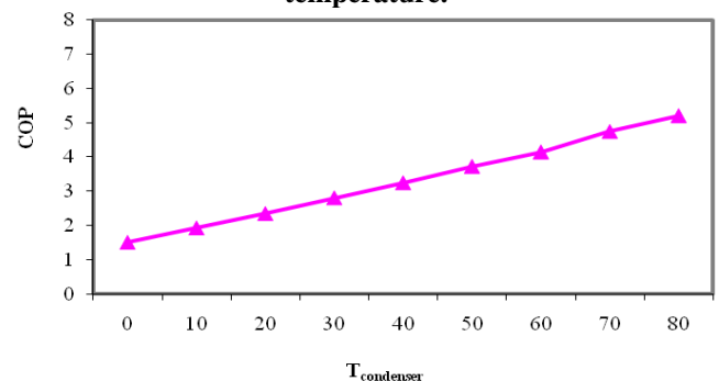
Figure 7. Heat pump performance vs condensation temperature.
