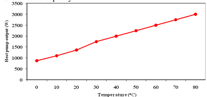
Figure 20. Variation of heat pump output with temperature.
