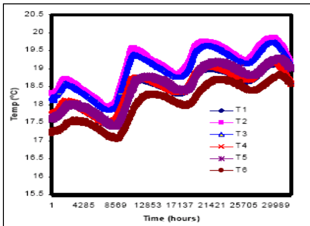
Figure 19. Variation of temperatures for heat exchanger for year.
