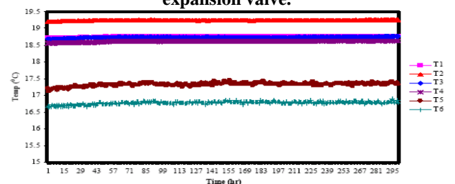
Figure 17. Variation of temperatures for heat exchanger for two weeks.
