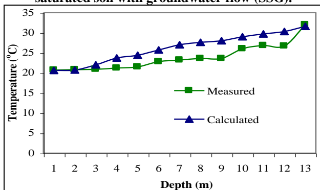
Figure 11. Comparison of calculations and experiments for saturated soil without groundwater flow (SS).
