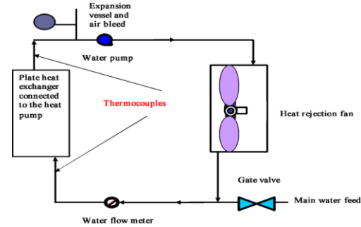
Figure 1. Sketch of installing heat pump.
