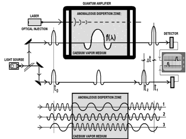
Figure 5. Experiments of L. Wang - superluminal light propagation
