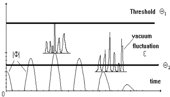
Figure 4. Quantum measurements.
