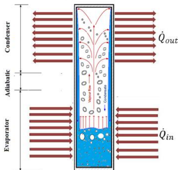
Figure 1. Gravity-assisted wickless heat pipe (two-phase closed thermosyphon).
