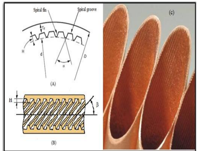
Figure 4. Thermosyphons with grooved inner surface
