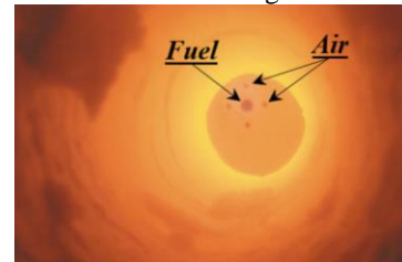
Figure 5. uniform volume combustion and low temperature flame, adapted from [15].
