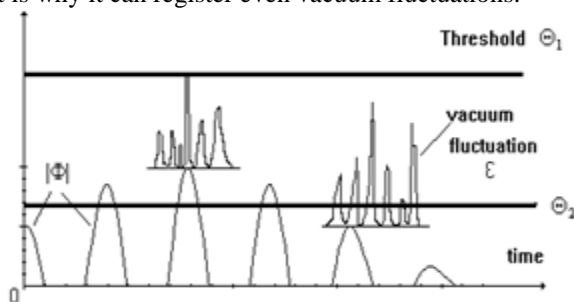
Fig.4. Quantum measurements.
