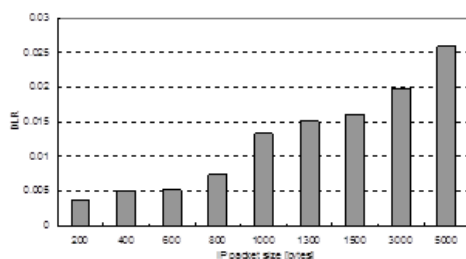
Fig. 3. Datagram Loss Rate(DLR) in terms of IP datagram size after mobile transmission.
